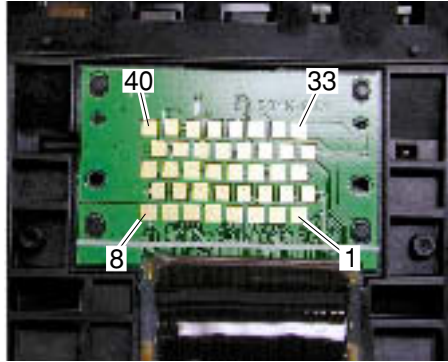
Figure 4-12 Print Head
