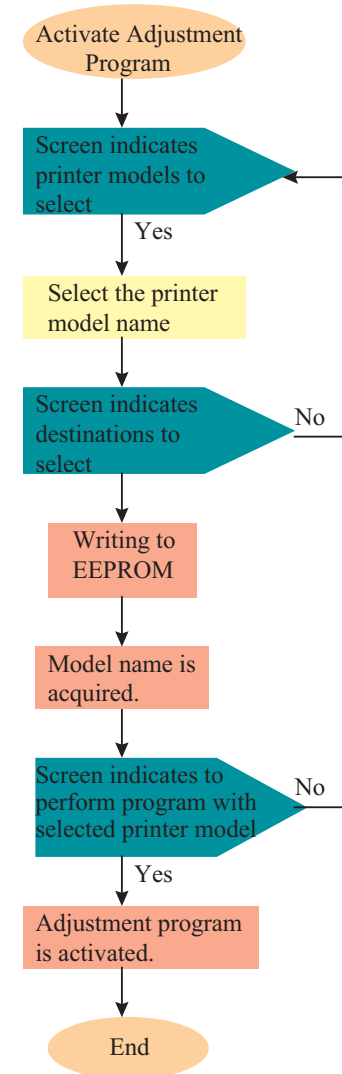
Figure 5-1. Flow Chart
