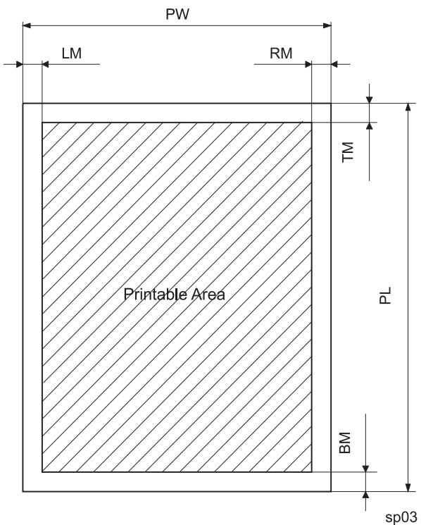
Figure 1-1. Printable Area
